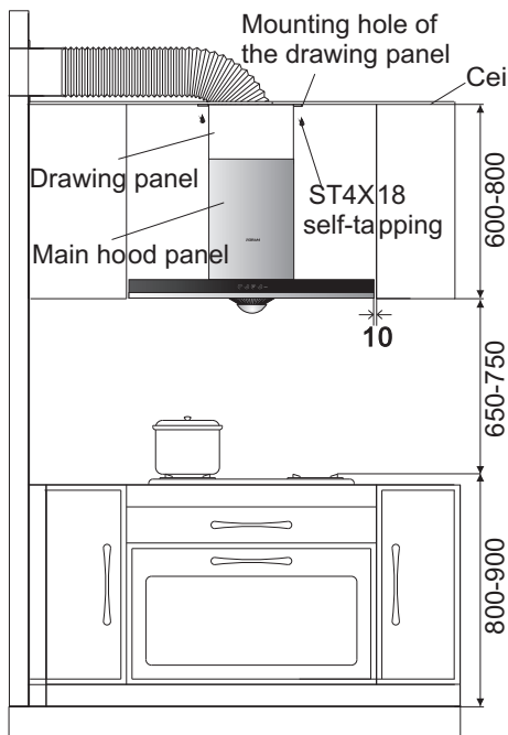
(Figure 1-1 Installation method of hood without removable baffle)
